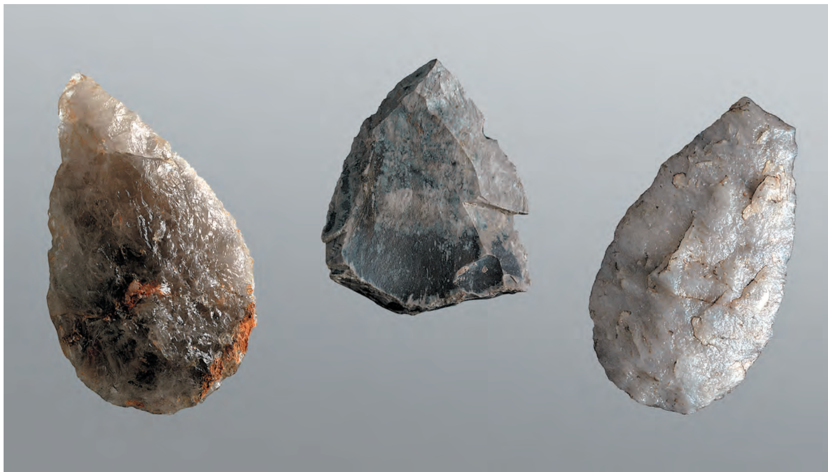
Fourth Cataract Survey, Middle Palaeolithic projectile points recovered from the Wadi Umm Rahau
